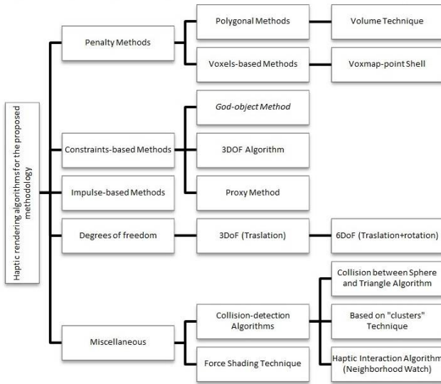
Figure 3. Classification of Haptic Rendering Algorithms.
