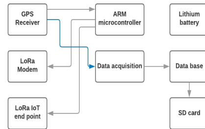
Figure 4. Balloon's payload block diagram
