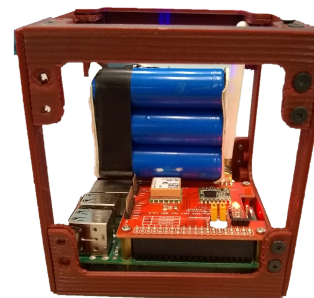
Figure 5. Balloon's payload
