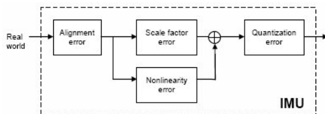
Figura 4. IMU Faulty Model.
