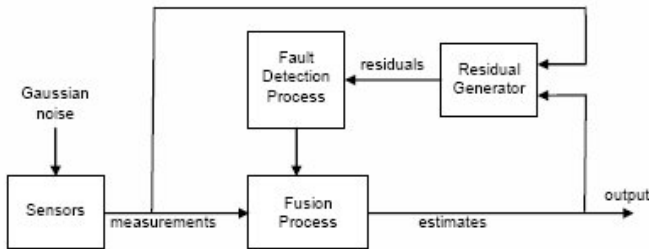
Figure 5. Adaptive Sensor Fusion System.
