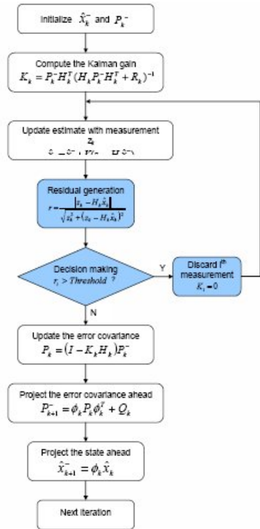
Figure 6. Adaptive Sensor Fusion Architecture Flow Chart.
