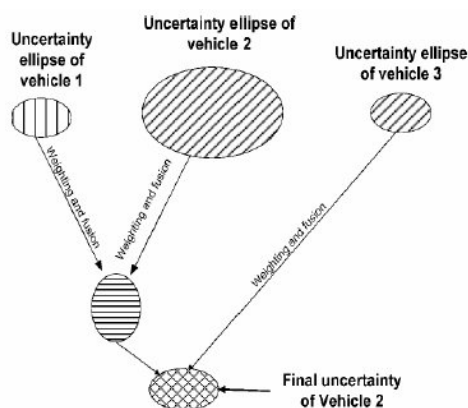
Figura 8. Principle of geometric data fusion approach in collaborative positioning of vehicles.
